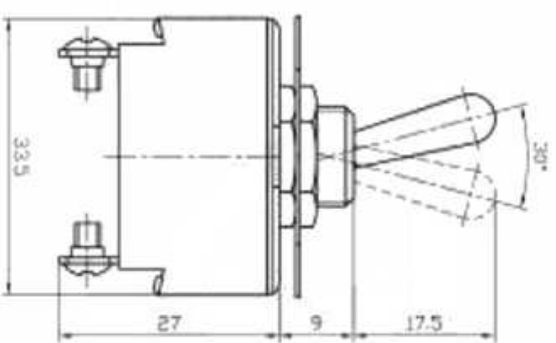
Outline Drawing
